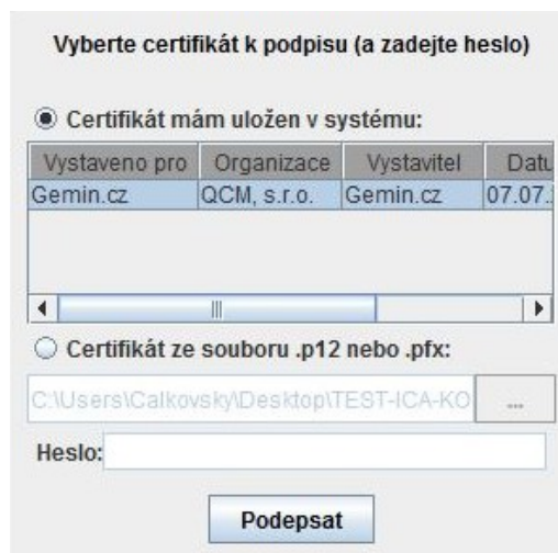
Figure 7: “Signer” applet
