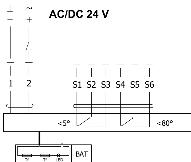
Servopohon BELIMO BFL 24-T(-ST)
